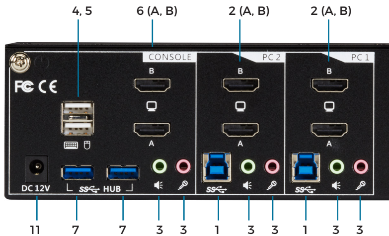
FIGURE 2-2. BACK PANEL OF THE KV6222H
