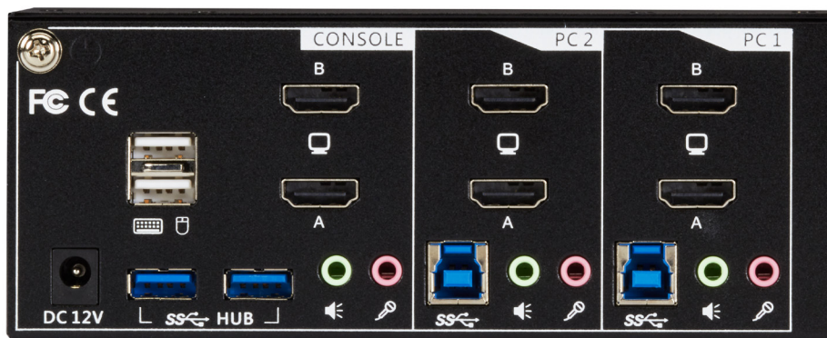
FIGURE 3-1. KV6222H - REAR VIEW
