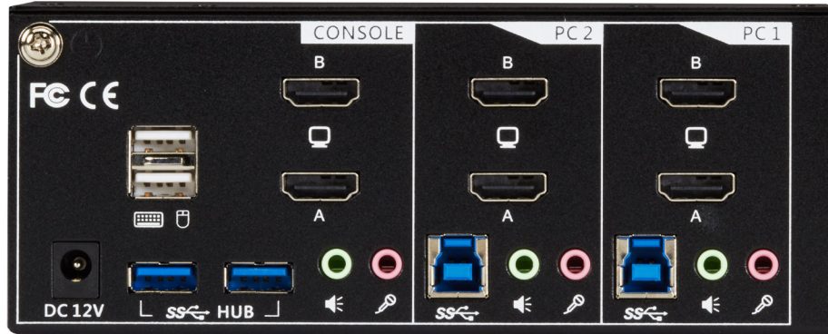
FIGURE 3-1. KV6222H - REAR VIEW
